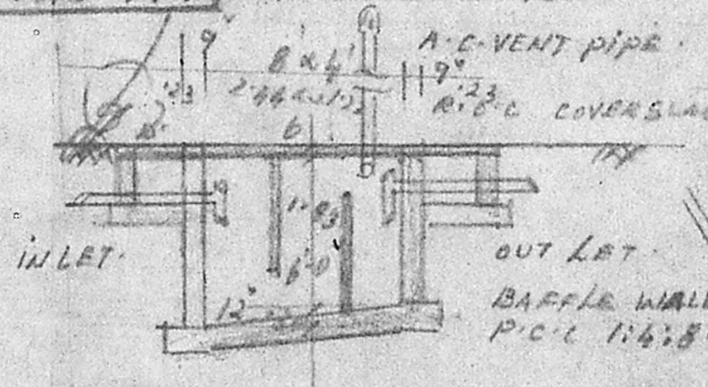
SECTION OF SEPTIC TANK SECTION OF WELL
