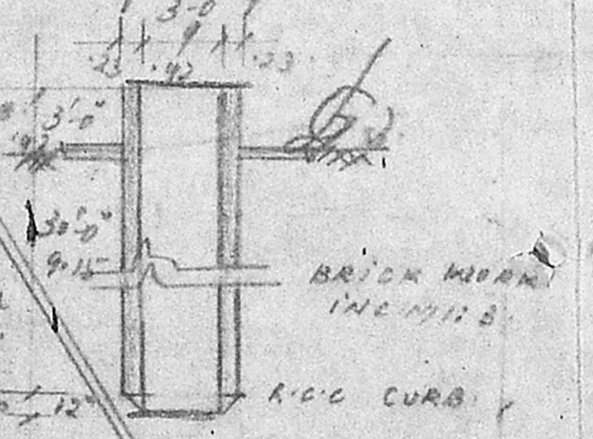
SECTION OF SEPTIC TANK SECTION OF WELL
